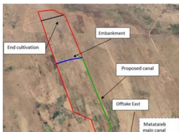
Figure 15. general layout of the intervention illustrating the locations of the embankment and proposed canal
