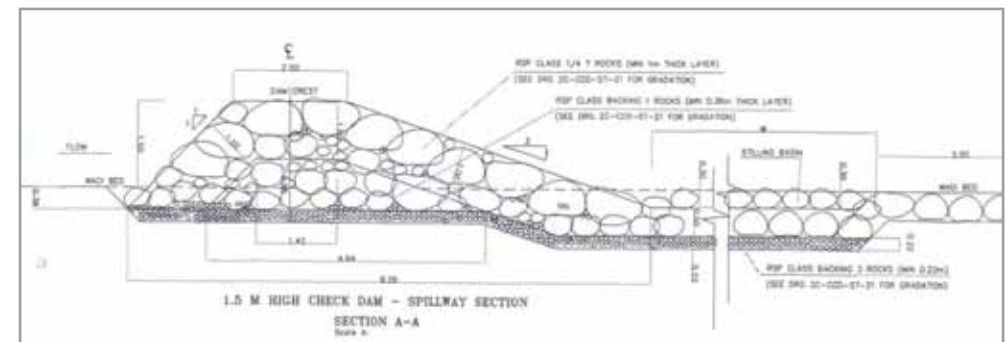
Figure 2: Features of a cross section of a 1.5 m high check dam at wadi Qaradha, Yemen
