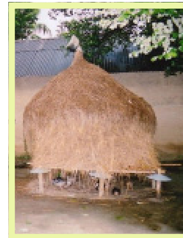
Figure 17: Example of rotational disk at the poles to prevent rats to climb up
