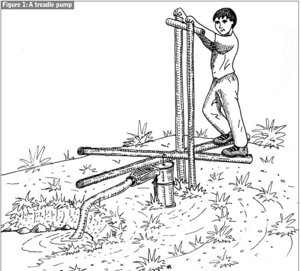
Figure 1: A treadle pump
