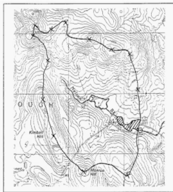
Figure 2.1 Delineating a water catchment
